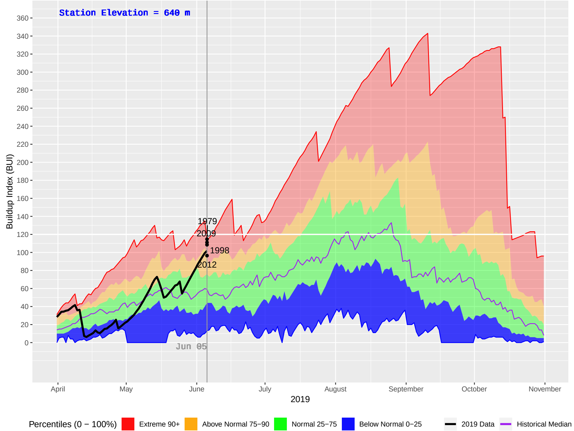
TURTLE (286) : Historical (1977–2018), Current (2019) Daily Buildup Index (BUI)
