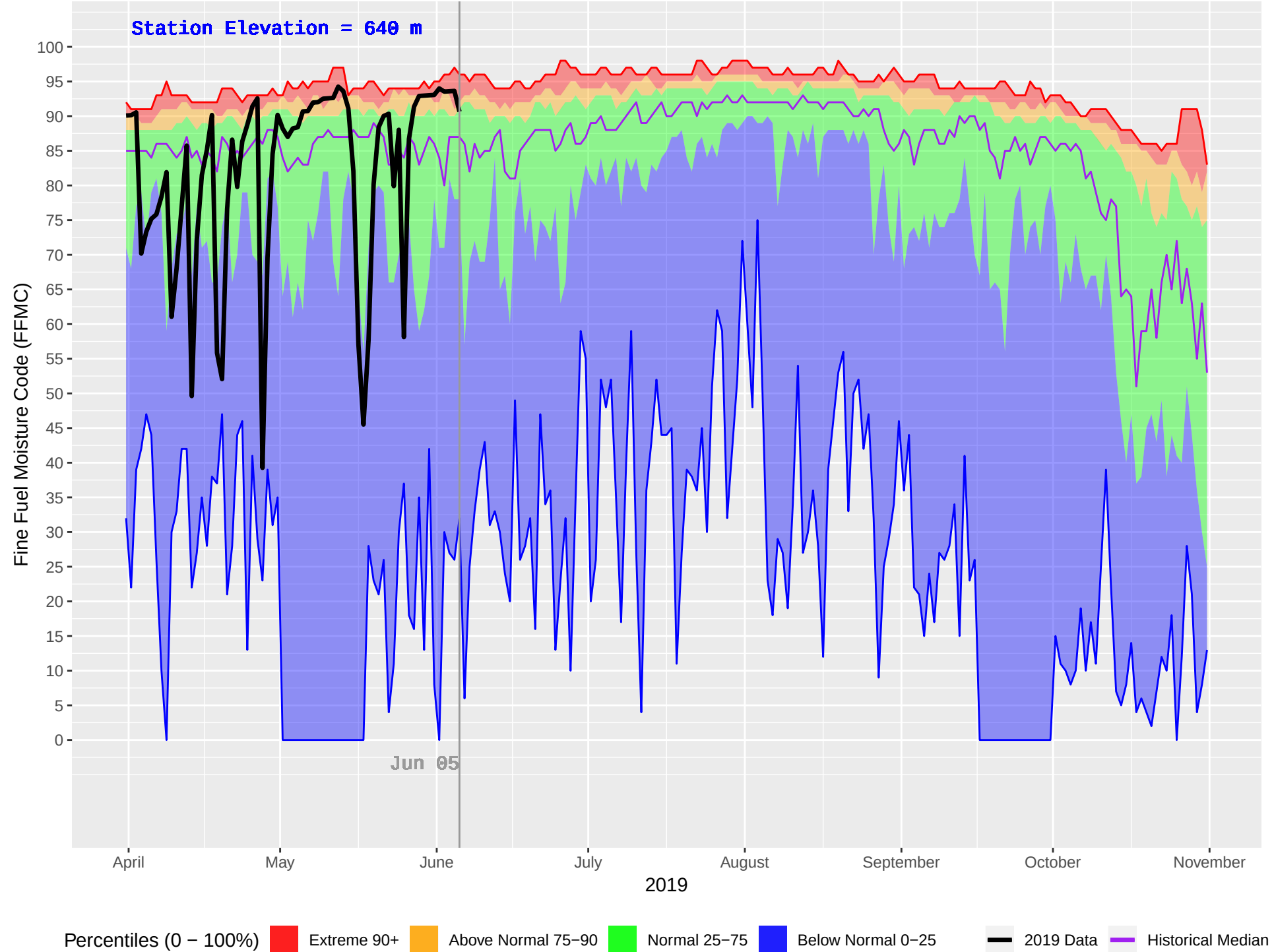
TURTLE (286) : Historical (1977–2018) and Current (2019) Daily Fine Fuel Moisture Code (FFMC)
