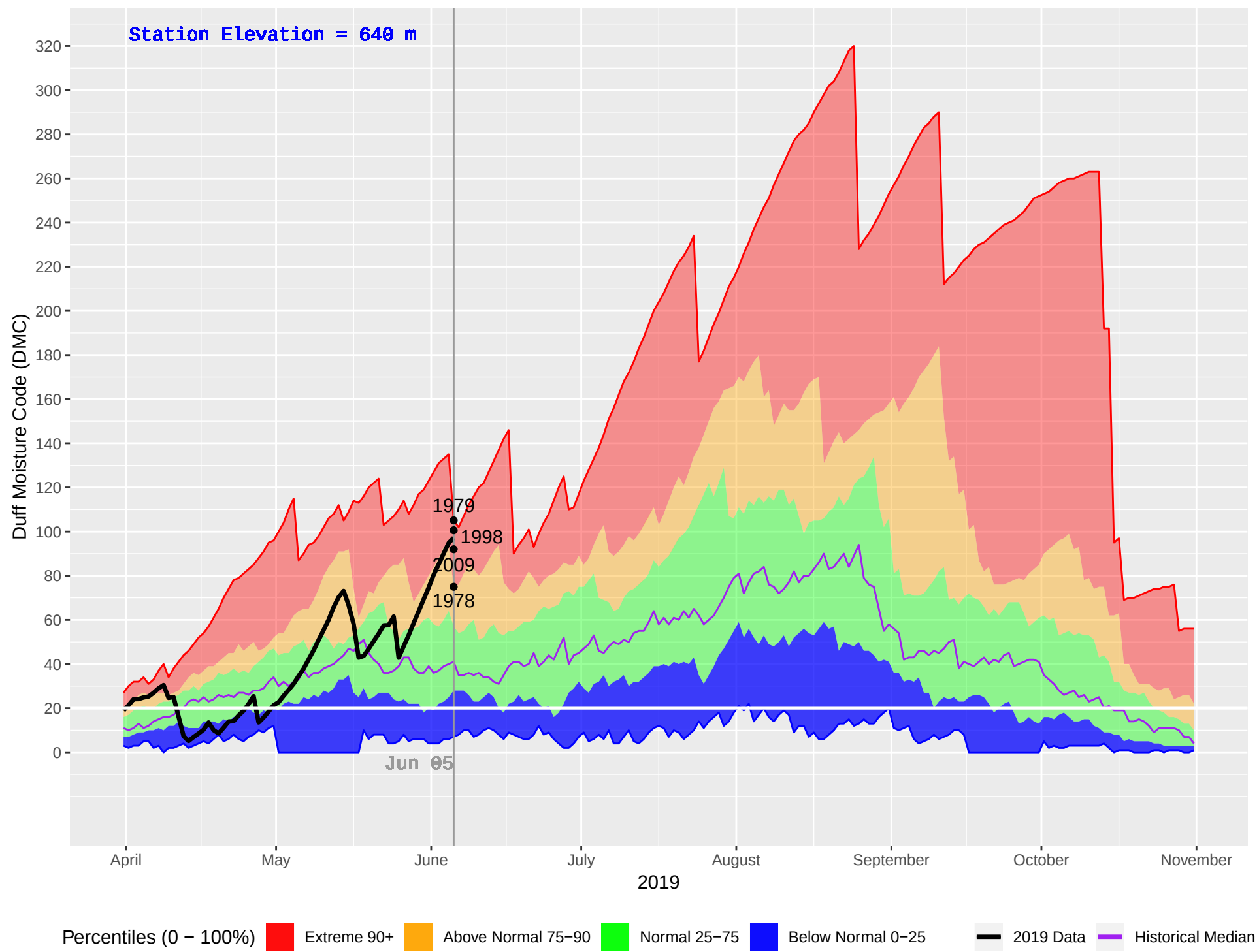
TURTLE (286) : Historical (1977–2018), Current (2019) Daily Duff Moisture Code (DMC)
