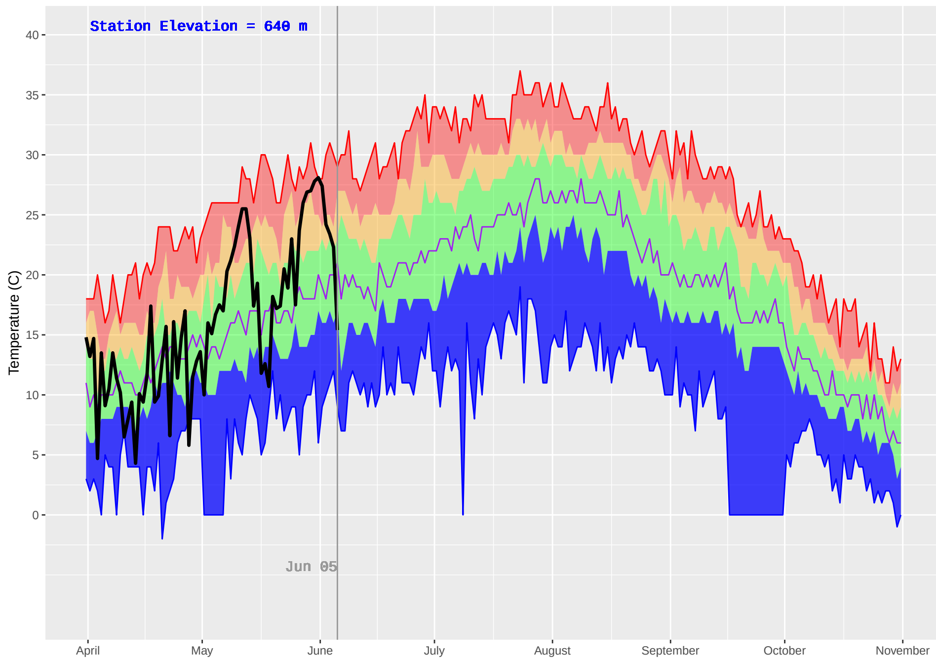
TURTLE (286) : Historical (1977–2018) and Current (2019) Daily Temperature
