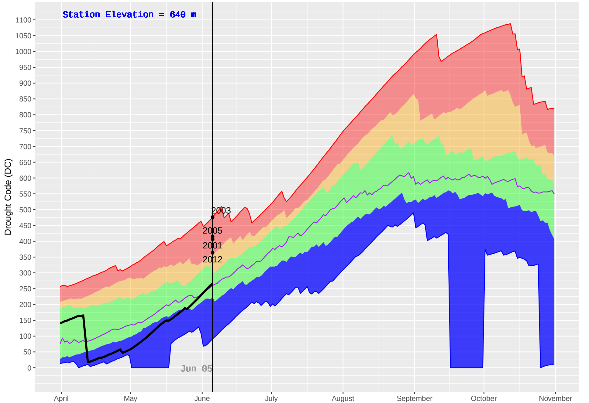
TURTLE (286) : Historical (1977–2018) and Current (2019) Daily Drought Code (DC)
