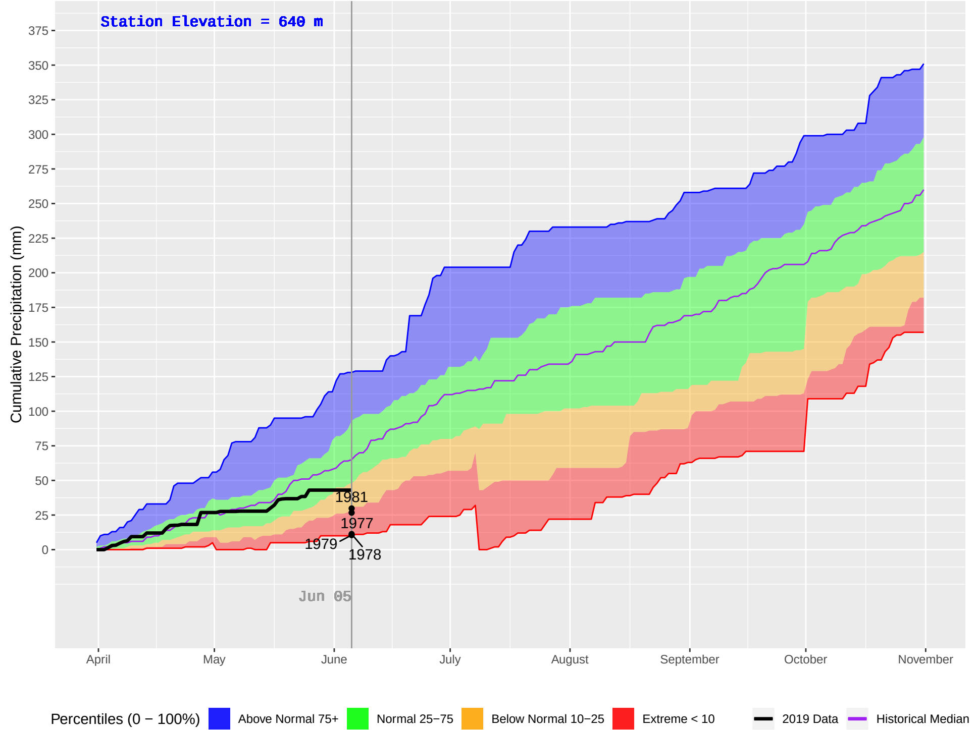
TURTLE (286) : Historical (1977–2018), Current (2019) Daily Cumulative Precipitation
