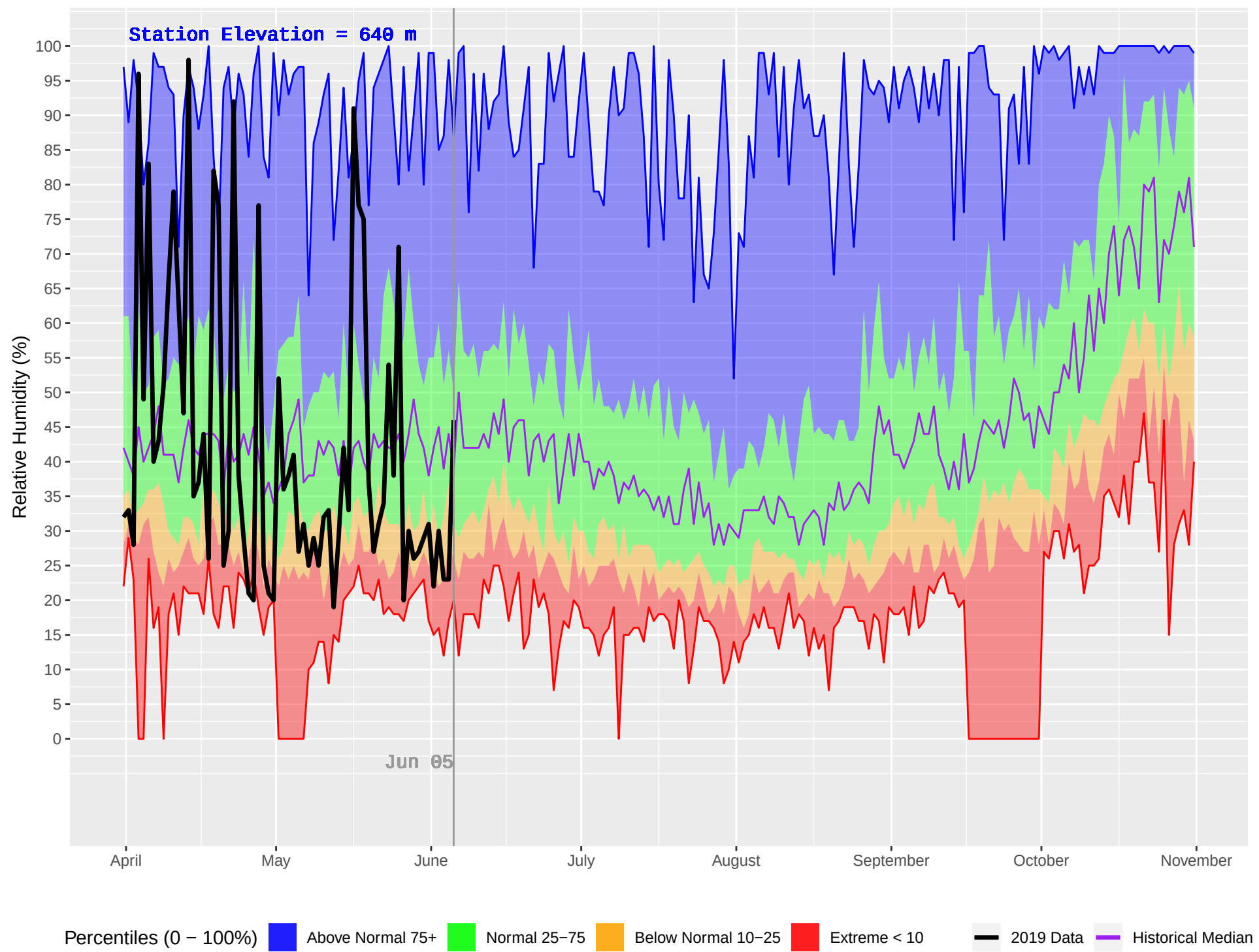
TURTLE (286) : Historical (1977–2018) and Current (2019) Daily Relative Humidity
